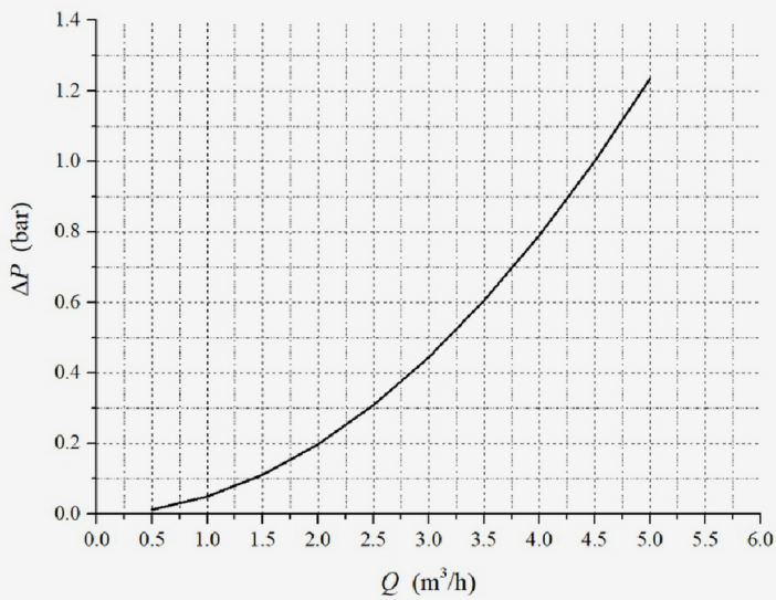
Two-Way Valve Characteristic Curve
